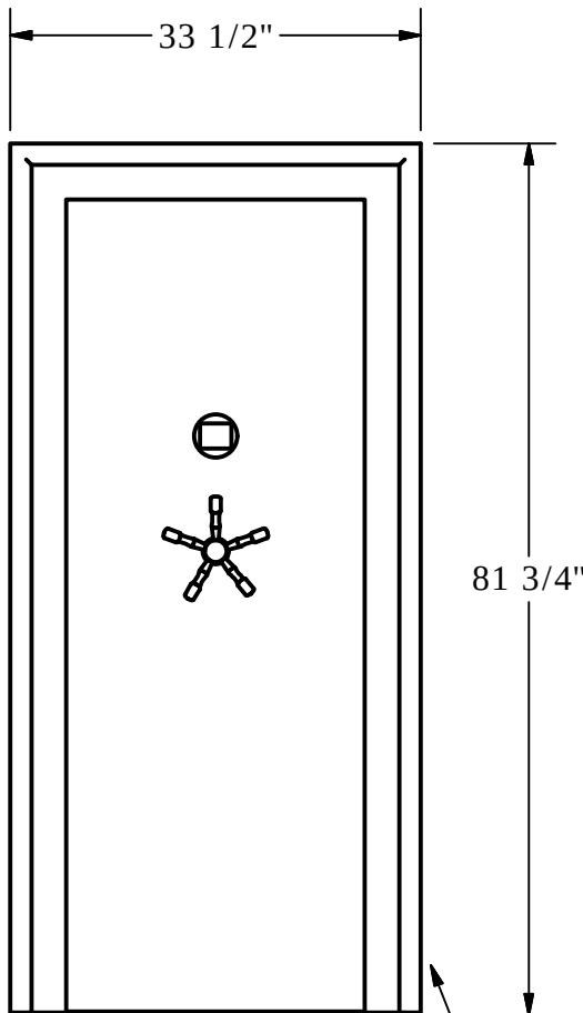
Front View
